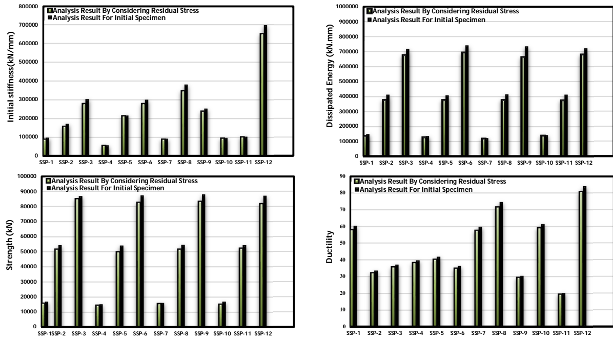
Fig. 4. The effect of residual stress on the performance of corrugated shear panels
