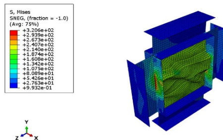
Fig. 3. Deformation and distribution of Von-Mises stress distribution of the SSP-6 shear panel model under the applied cyclic loading
