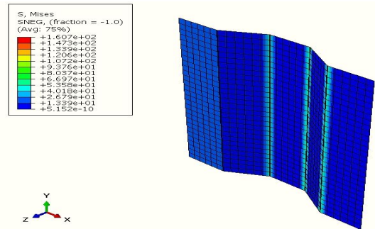
Fig. 1. The distribution of the Von-Mises stress in the corrugated steel panel after the bending process
