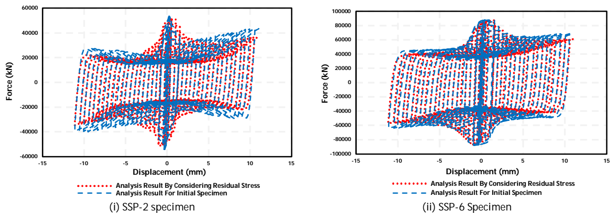
Fig. 2. Force-Displacement diagram of two specimens
