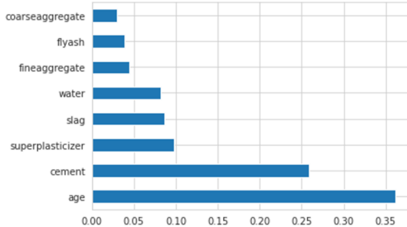
Fig. 1. Feature importance analysis
