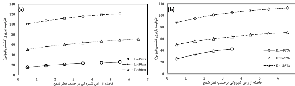
Fig. 1 Comparison of response of pile groups
