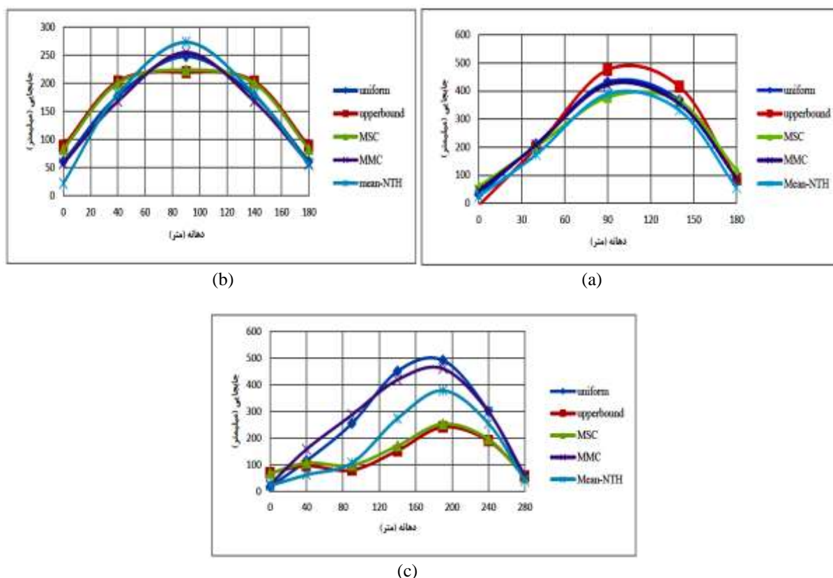
Fig 2. Deformation pattern prediction, (a) Group 111 bridge, (b) Group 123 bridge, and (c) Group 11233 bridge
