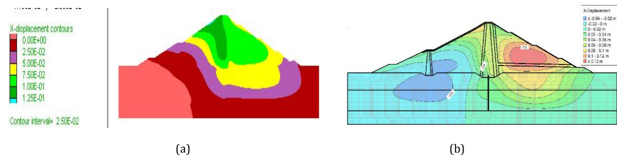
Fig. 2. a) Horizontal displacement before impounding in FLAC software, b) Horizontal displacement after impounding in Geo studio software
