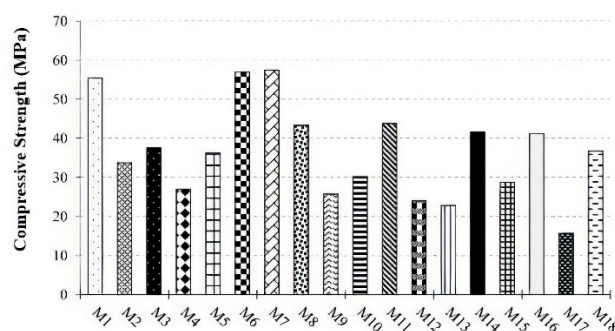
Fig. 1. Compressive strength of mortars
