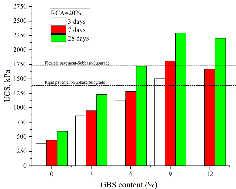
Fig. 3. UCS of clay-20%RCA mixture with GBS different content at different curing times, and limits of UFC for subgrade stabilization
