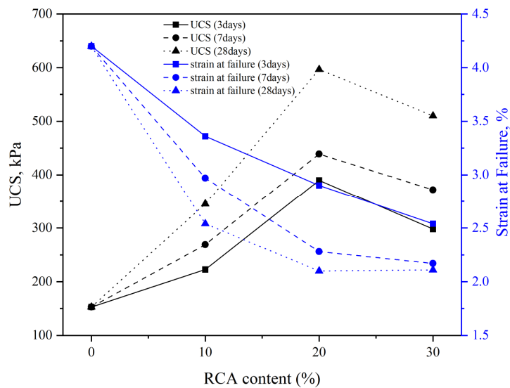
Fig. 2. UCS and strain at failure for soils with different percentages of RCA
